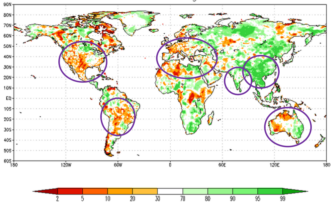
Calculated Soil Moisture Ranking Percentile 20220515
