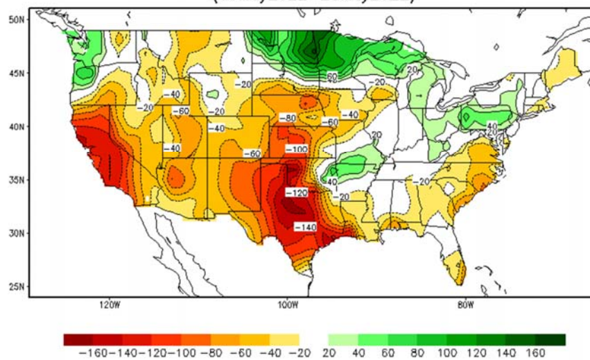
Predicted Soil Moisture Anomaly (mm) (16May2022–23May2022)
