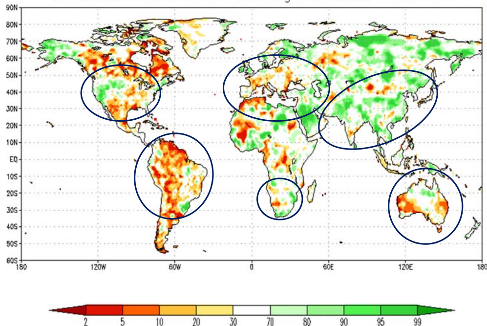
Calculated Soil Moisture Ranking Percentile 20231018
