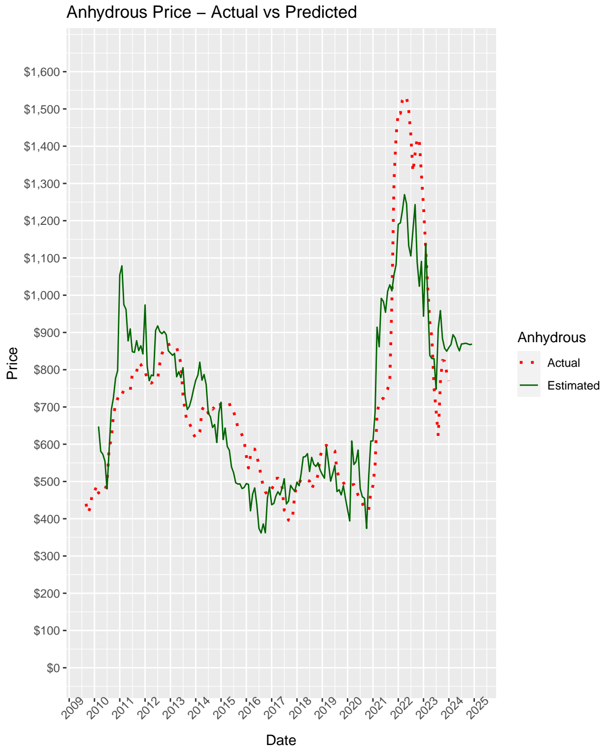
Figure 4: Actual Anhdrous Price vs Predicted Price - Long Term
