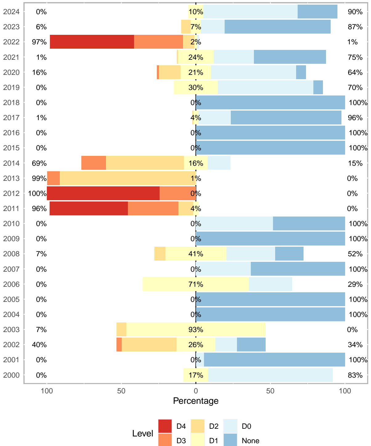
Figure 7: Southwest - Drought Conditions for Specific Week Since 2000
