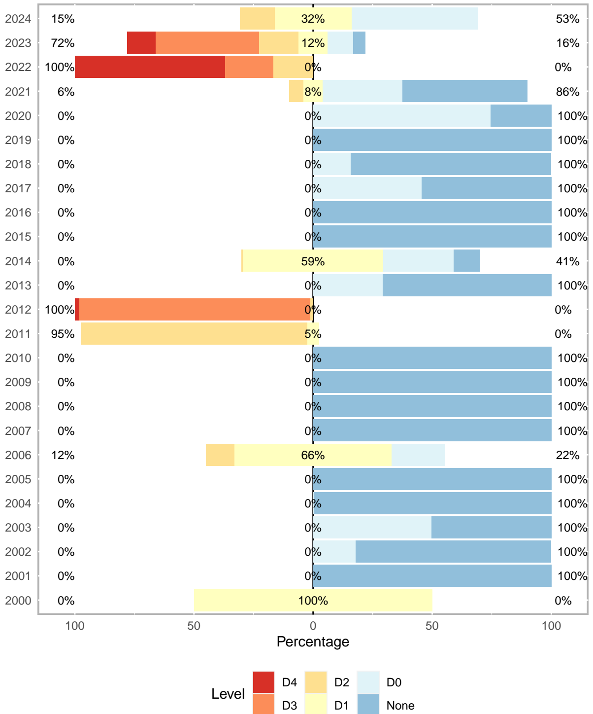
Figure 19: Southeast - Drought Conditions for Specific Week Since 2000
