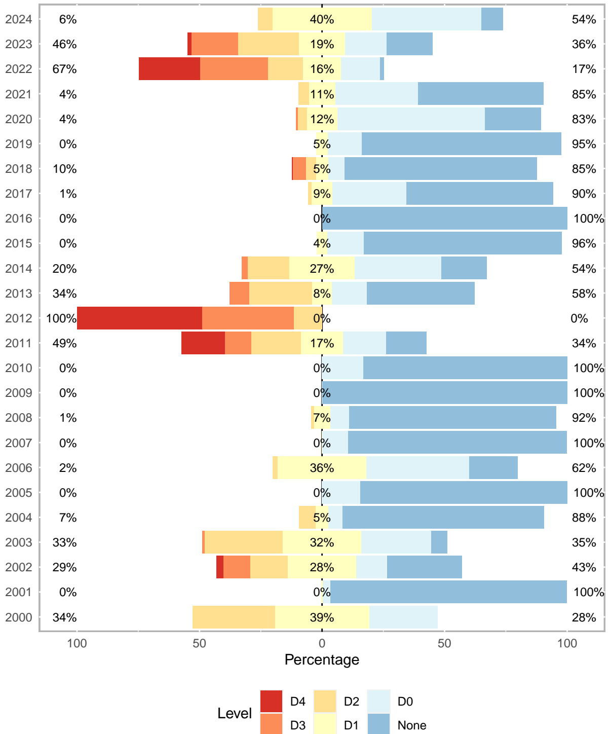
Figure 1: Kansas - Drought Conditions for Specific Week Since 2000
