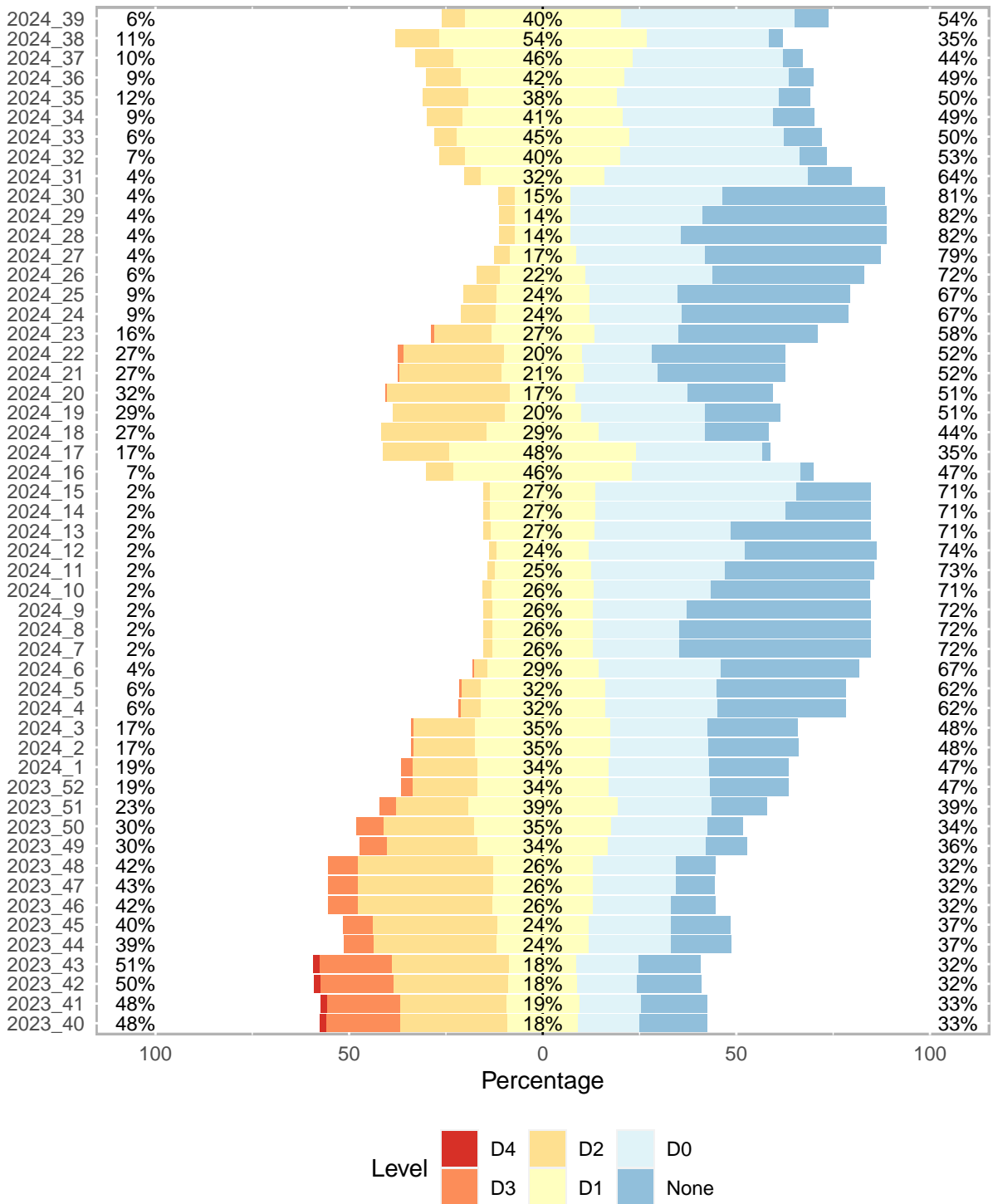
Figure 2: Kansas - Drought Conditions Each Week for Past Year
