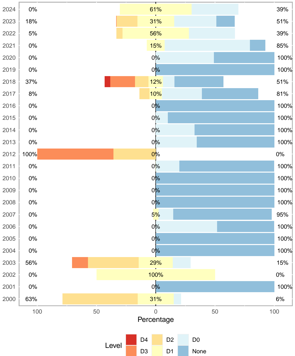
Figure 15: Northeast - Drought Conditions for Specific Week Since 2000
