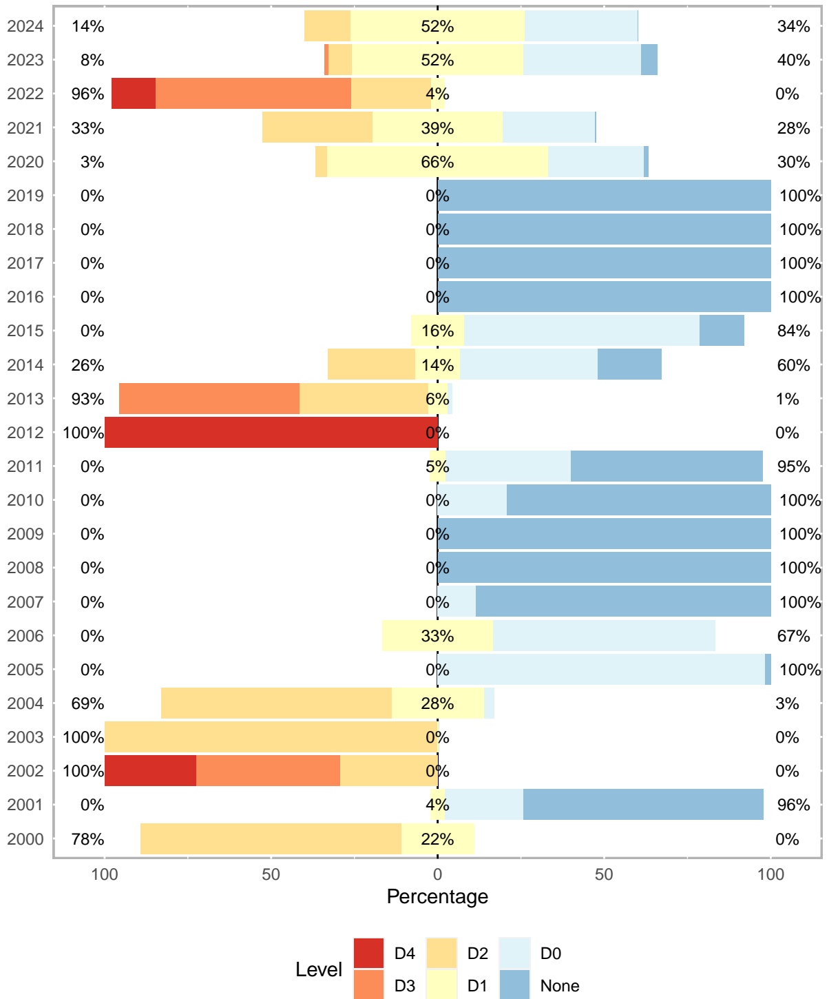
Figure 3: Northwest - Drought Conditions for Specific Week Since 2000
