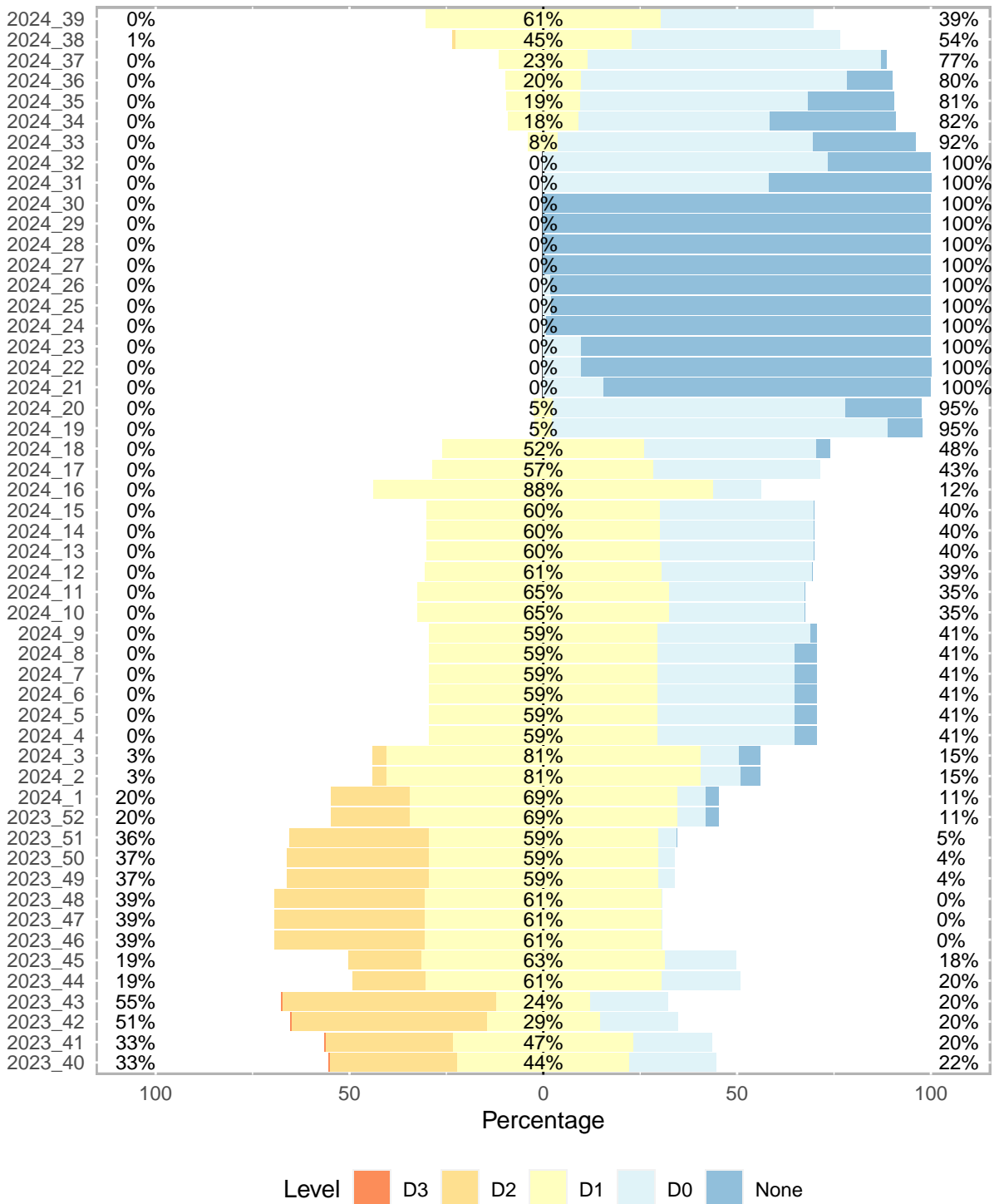
Figure 16: Northeast - Drought Conditions Each Week for Past Year
