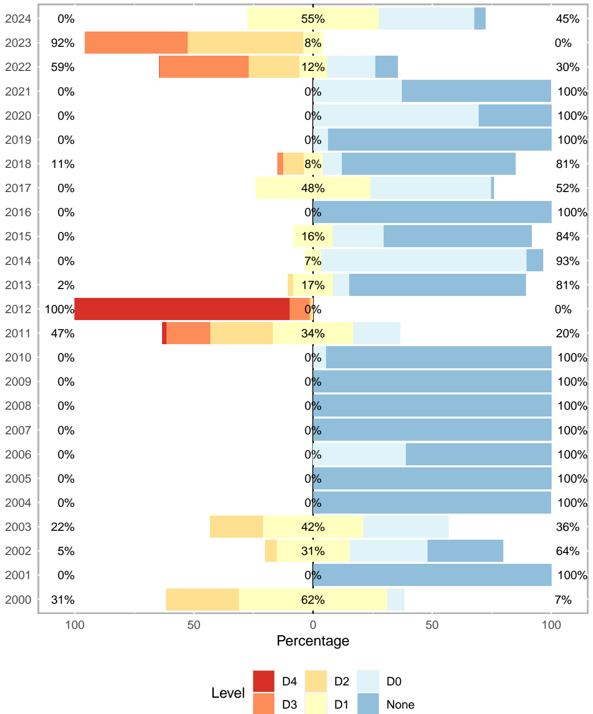
Figure 11: Central - Drought Conditions for Specific Week Since 2000
