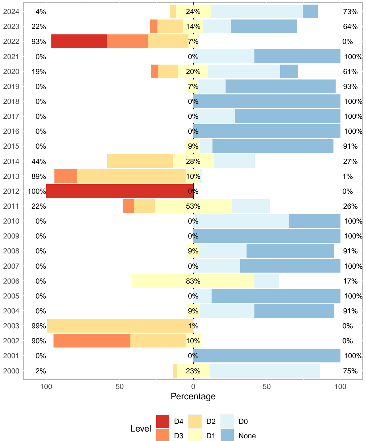
Figure 5: West Central - Drought Conditions for Specific Week Since 2000
