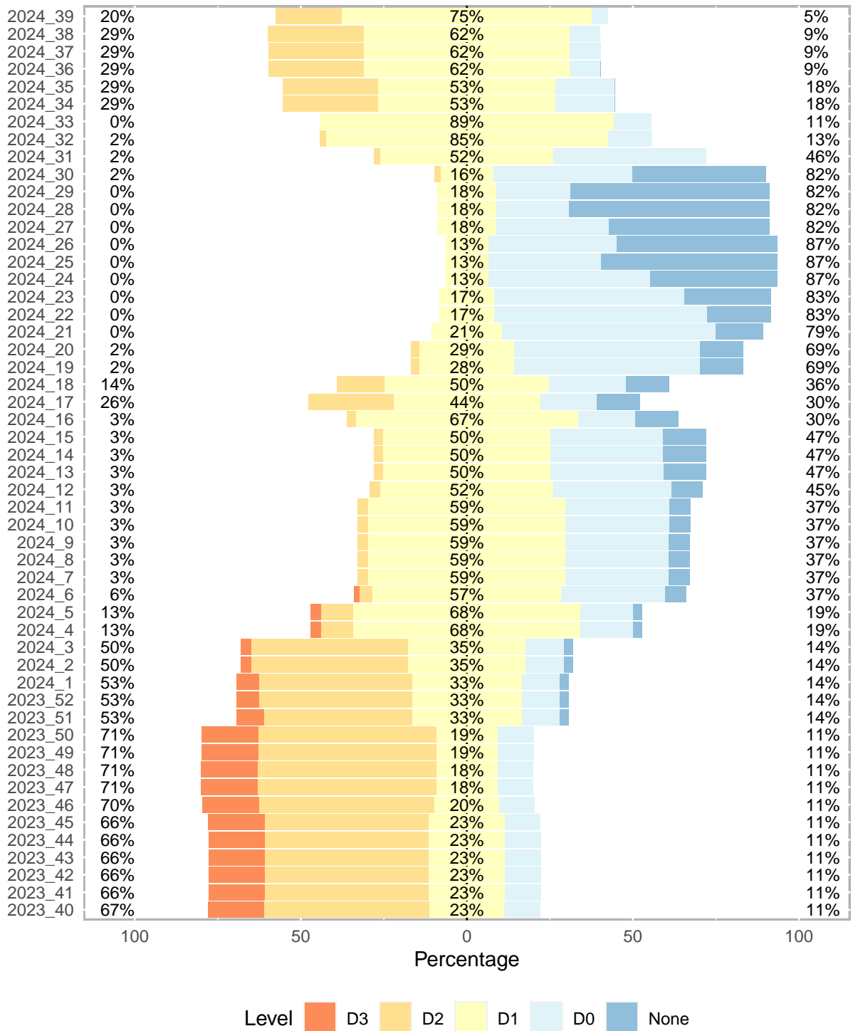
Figure 10: North Central - Drought Conditions Each Week for Past Year
