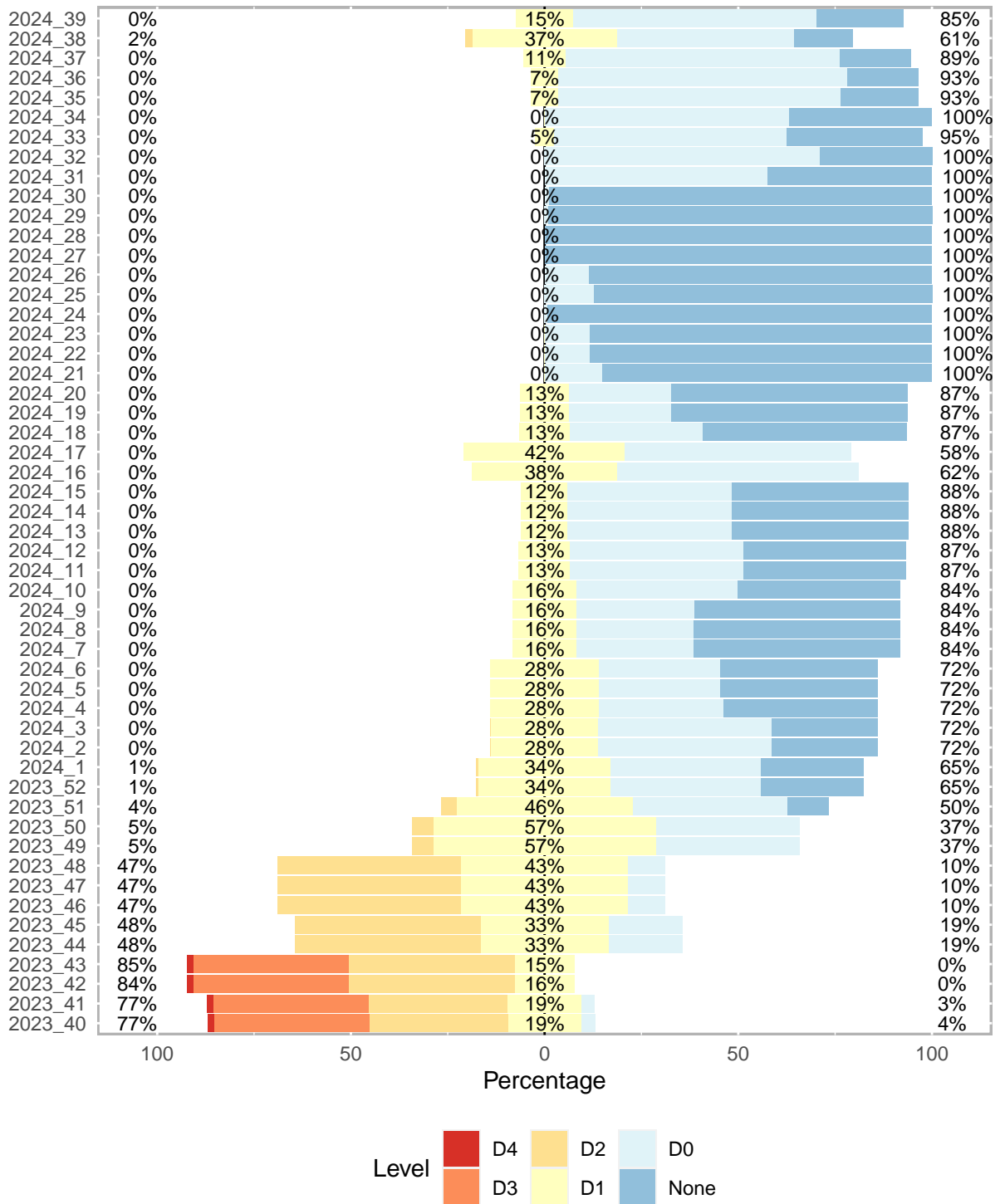
Figure 18: East Central - Drought Conditions Each Week for Past Year
