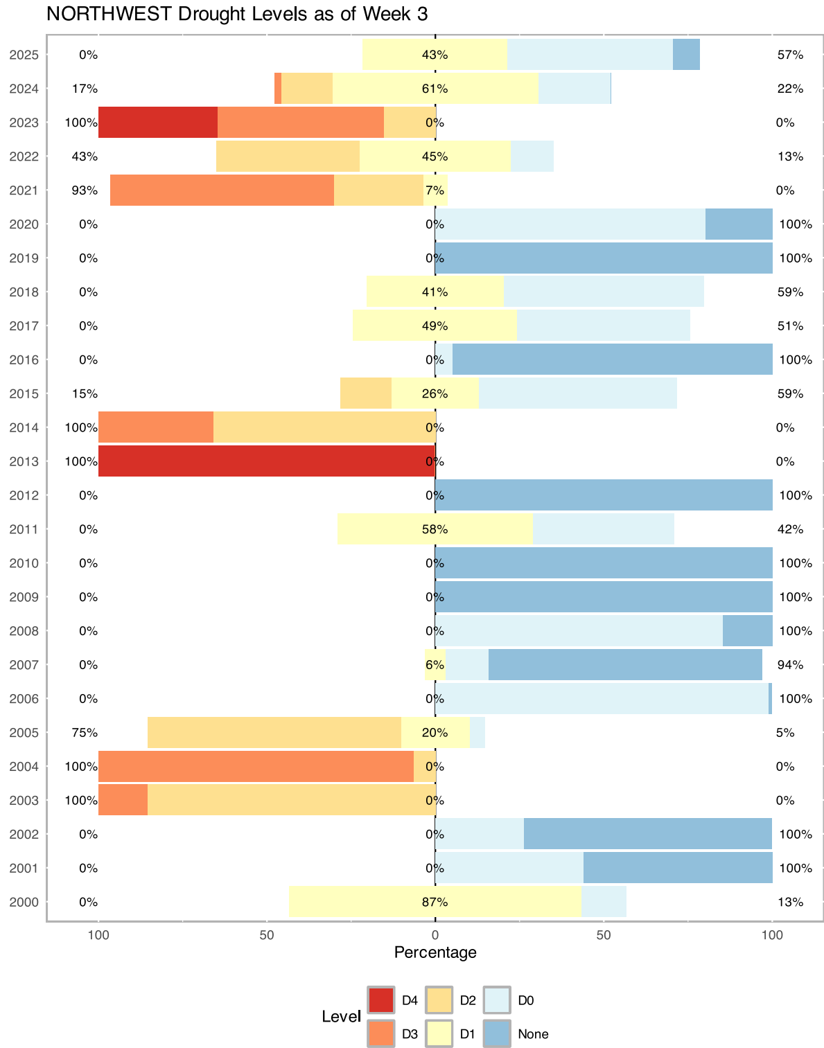
Figure 3. Northwest - Drought Conditions for Specific Week Since 2000
