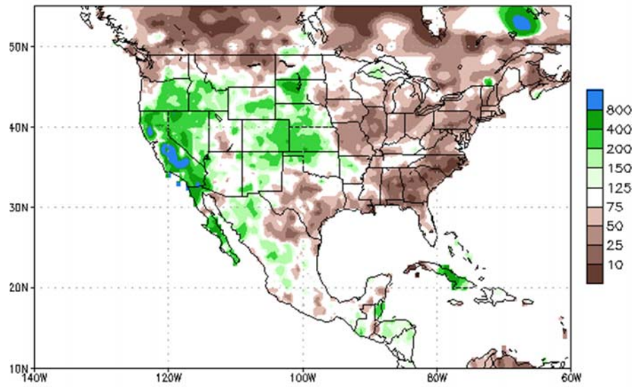
30-day Accumulated Precip % of Normal 25AUG2025-23SEP2025
