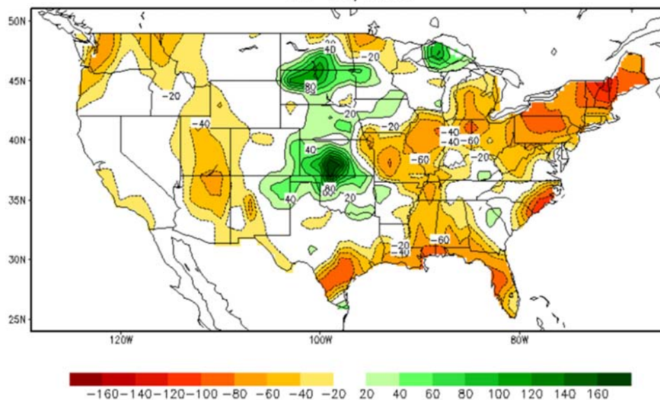
Calculated Soil Moisture Anomaly (mm) SEP 23, 2025
