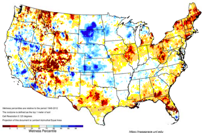
NASA GRACE-Based Root Zone Soil Moisture Drought Indicator September 22, 2025
