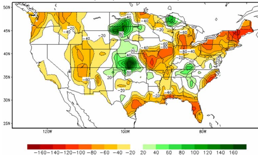
Predicted Soil Moisture Anomaly (mm) (24Sep2025-01Oct2025)
