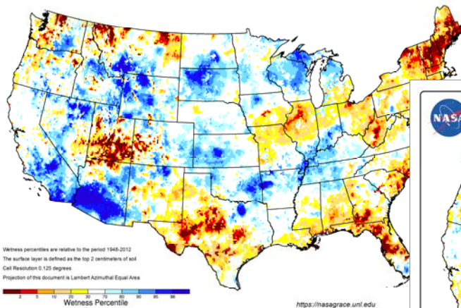
NASA GRACE-Based Surface Soil Moisture Drought Indicator September 22, 2025
